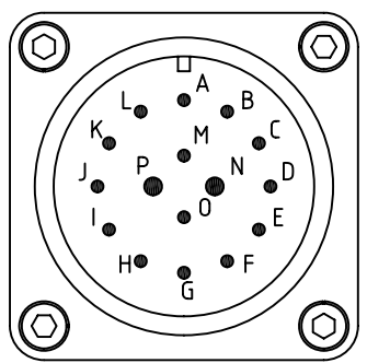
VIEW A SCALE 2.5X
